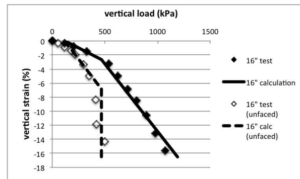
Figure 15 Transition at q_{ult} = WQ_{ult} (near 500 kPa) is validated for faced/unfaced pair of piers.
