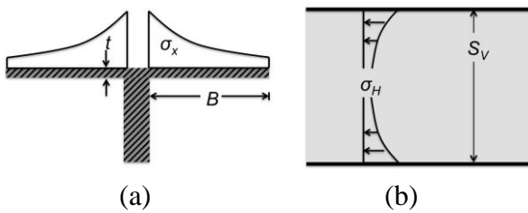
Figure 1 Shear lag in (a) beams is analogous to shear lag in (b) reinforced soil.
