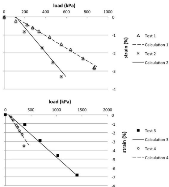
Figure 14 Calculations and measurements for four early pier tests, where load \leq q_{ult} = WQ
