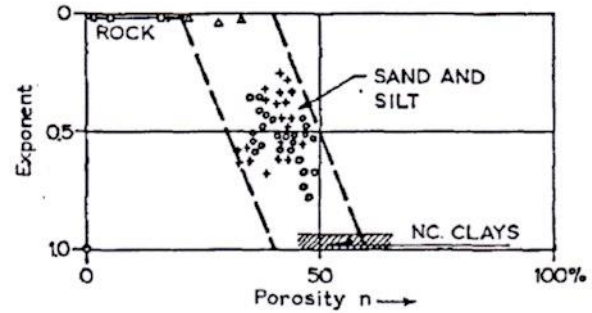
Figure 6 Janbu's data show that n \approx 0.5 for aggregates.
