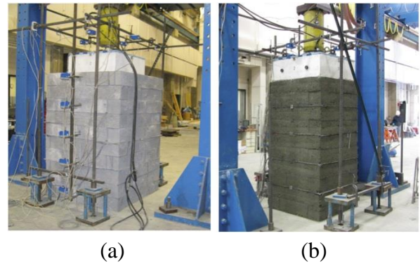
Figure 3 FHWA tested both (a) faced piers and (b) unfaced piers to ultimate capacity.
