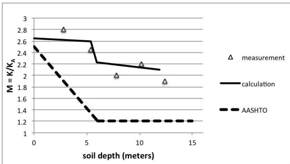
Figure 13 Measurements, calculations, and AASHTO's Simplified Method are compared for welded wire fabric wall WWI.
