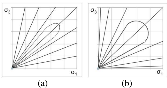
Figure 10 Compared to (a) Euclidean space, (b) stress space \sigma_1 - \sigma_3 distorts geometry.
